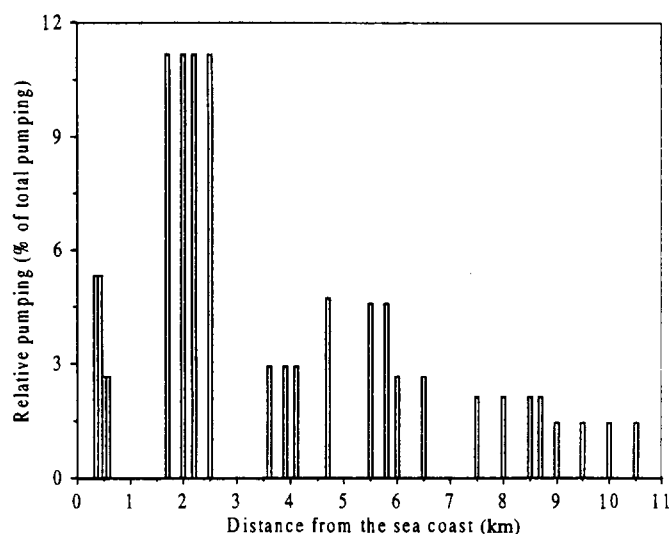
Figure 7 Relation between relative pumping and distance from the sea coast
