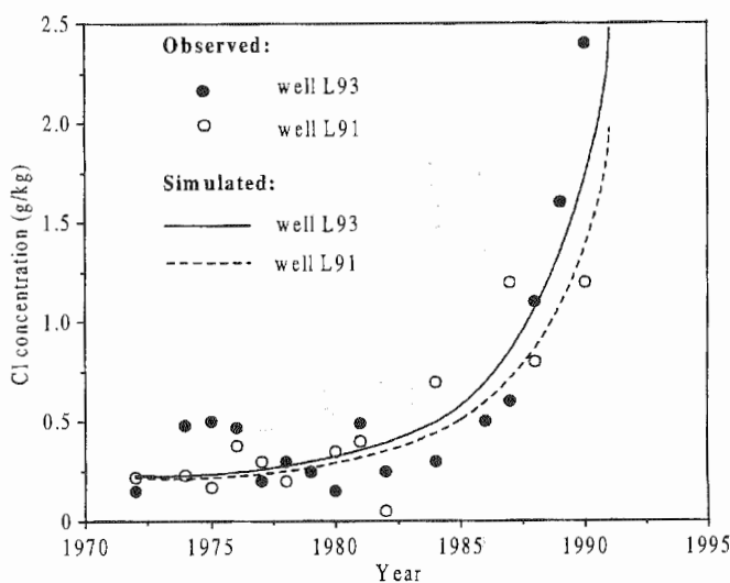
Figure 3 Observed and simulated Cl concentrations in two wells: well L91, 325 m from the sea coast, 10 m below the sea level; well L93, 300 m from the sea coast, 10 m below the sea level
