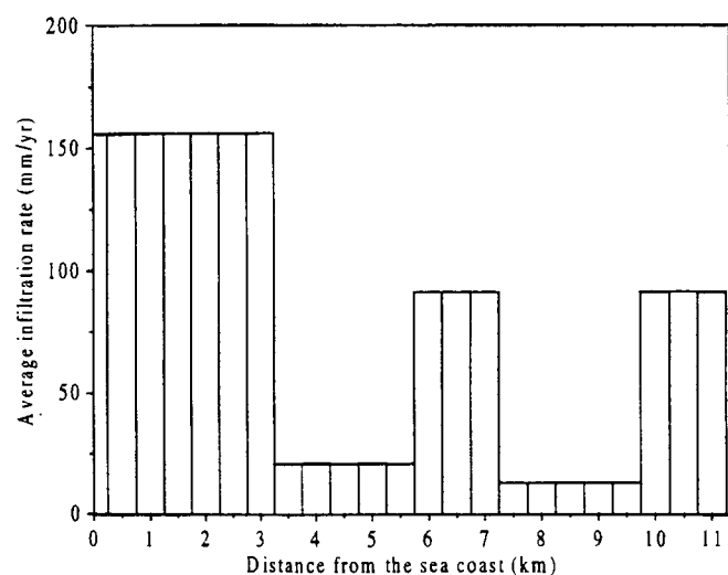
Figure 5 Relation between infiltration rate through the land surface and distance from the sea coast
