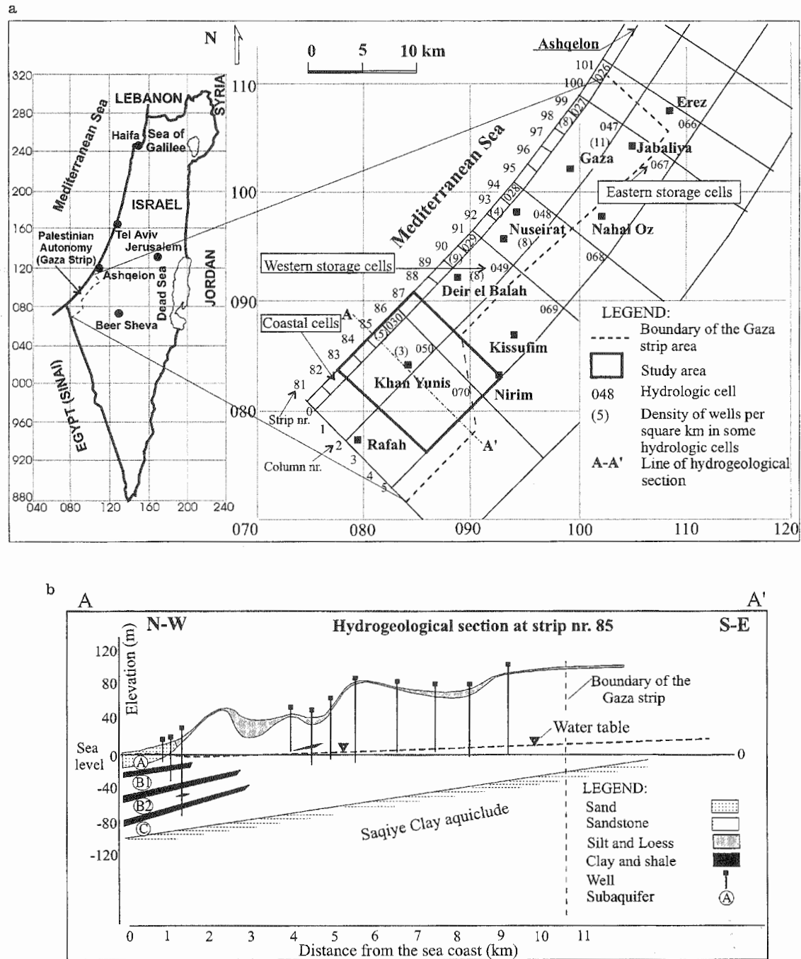
Figure 1 a Location and general map of the Gaza Strip showing study area and b section A-A'
